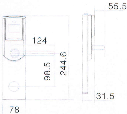
Front Panel
